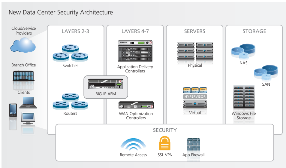
Figure 4: The new paradigm replaces stateful firewall services with BIG-IP LTM in the data center architecture.
